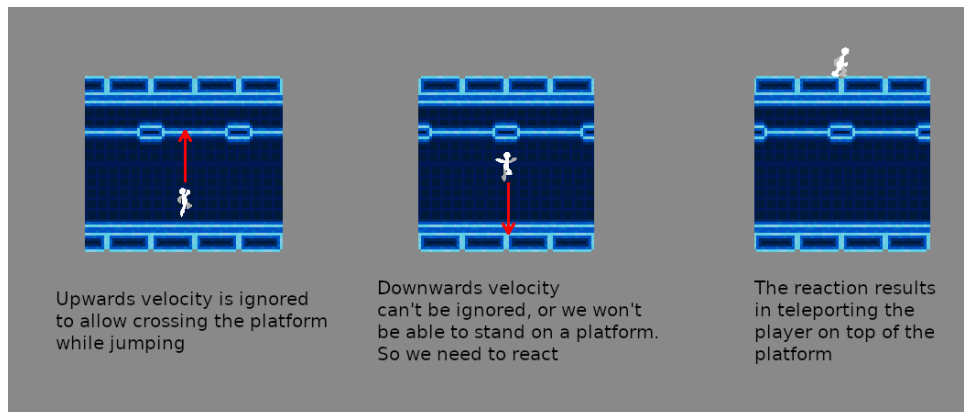
Figure 197: How velocity changing direction can teleport you
